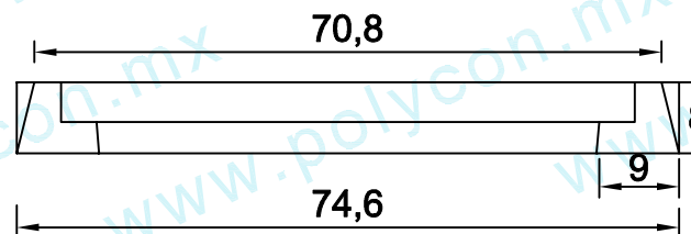
VISTA FRONTAL
