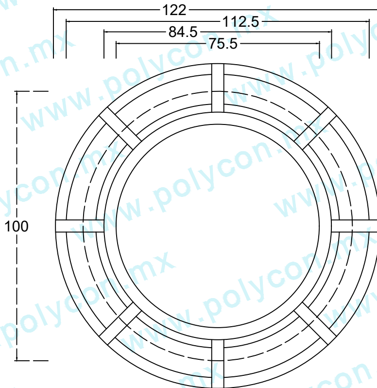
VISTA SUPERIOR BROCAL
